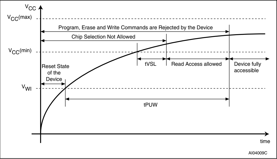
Figure 21. Power-up timing
