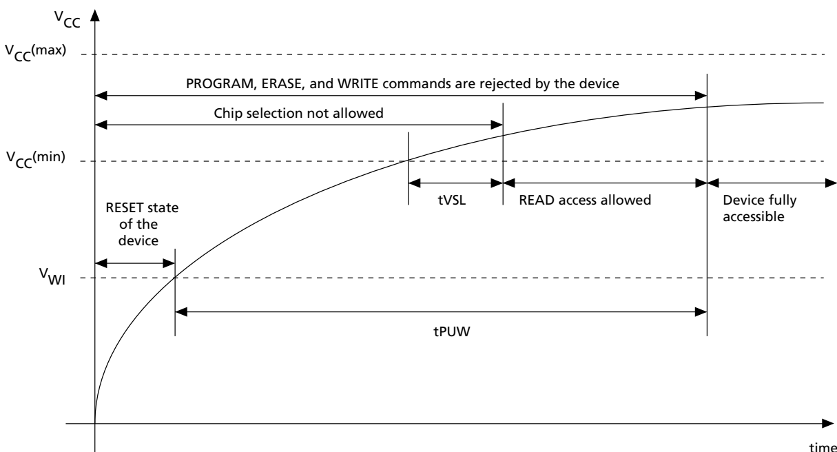
Figure 22: Power-Up Timing
