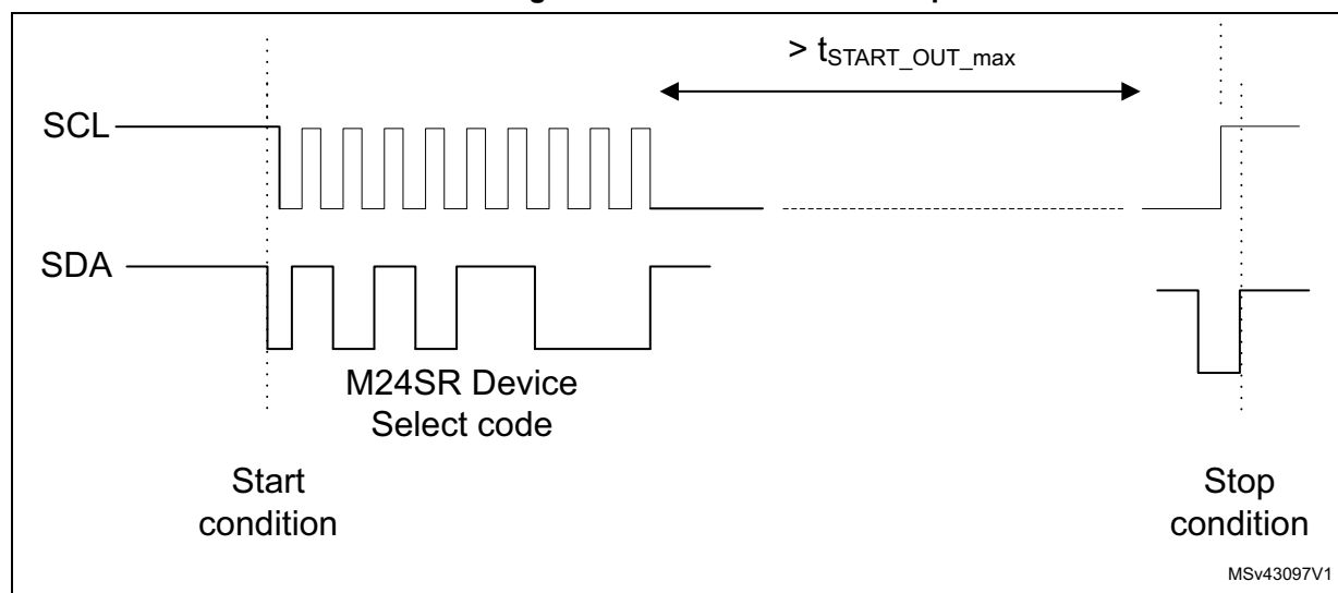
Figure 13. I 2 C token release sequence
