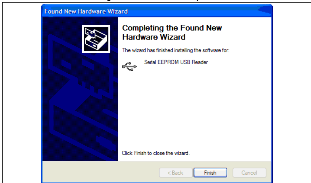
Figure 36. Installation complete
