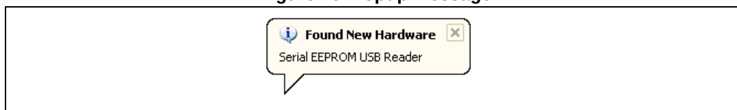
Figure 26. Popup message
