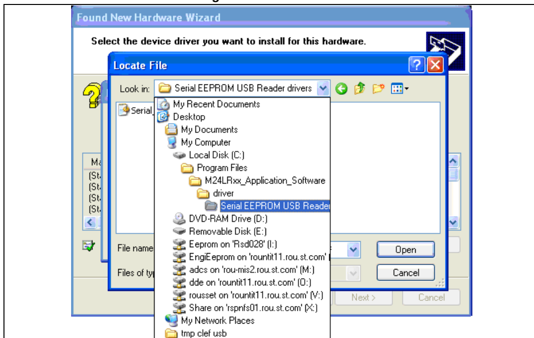
Figure 32. File location
