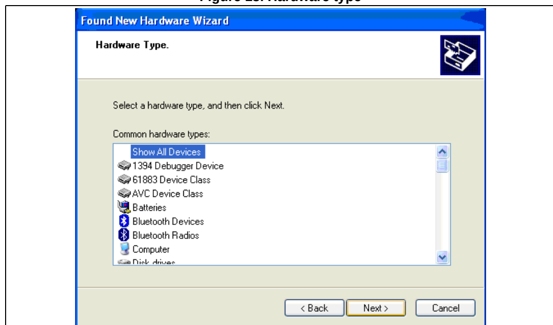
Figure 13. Hardware type
