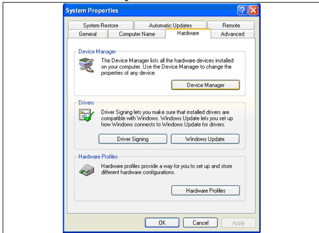
Figure 24. Hardware tab
