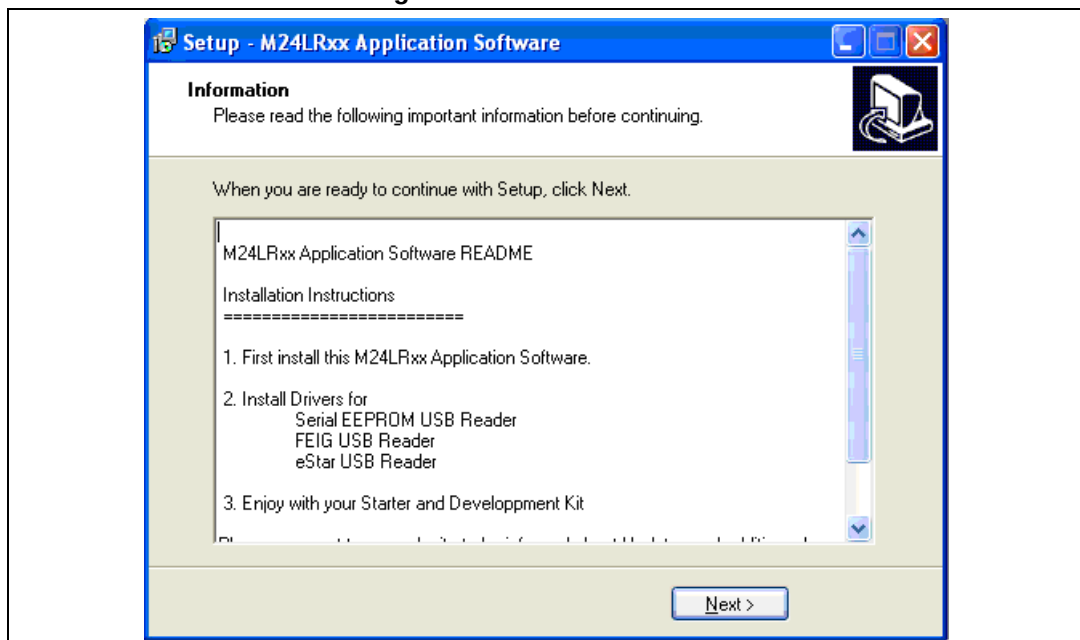
Figure 7. Software README
