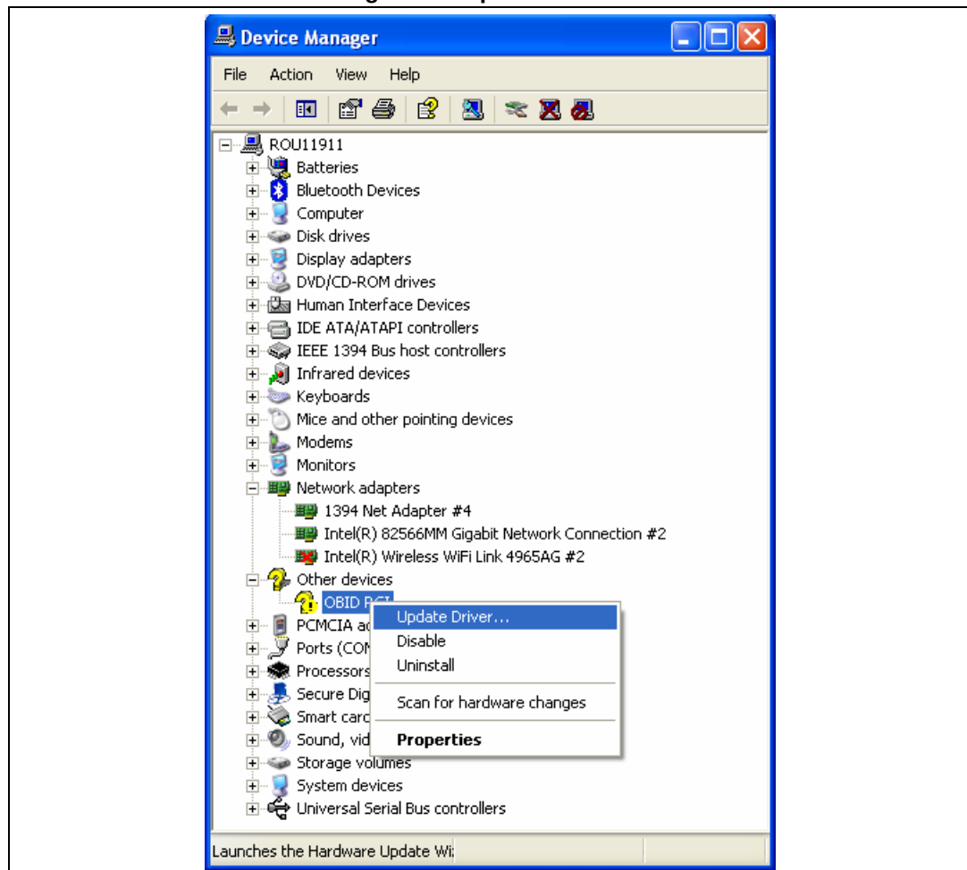
Figure 39. Update Driver...
