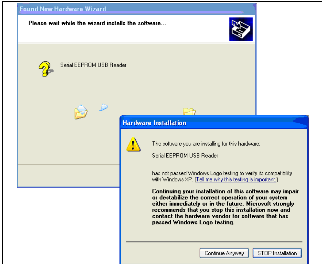
Figure 35. Software installation
