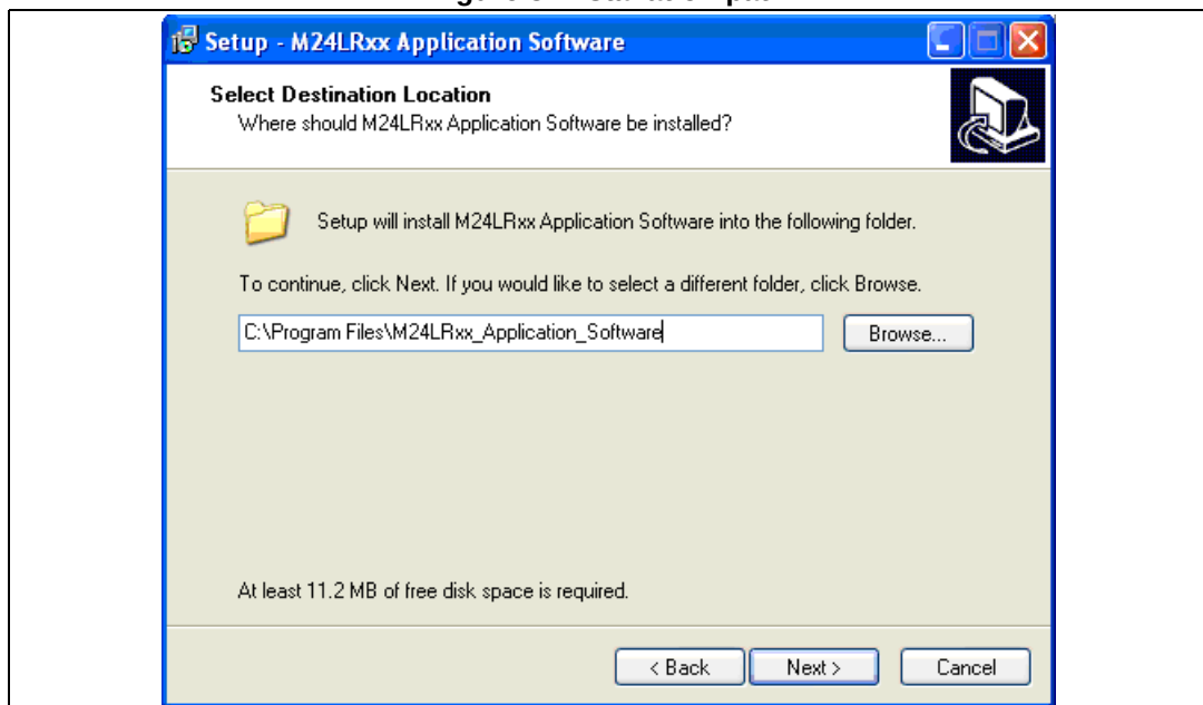
Figure 3. Installation path
