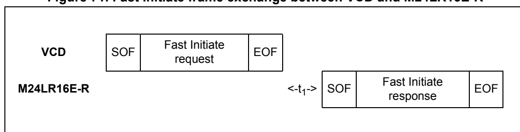
Figure 71. Fast Initiate frame exchange between VCD and M24LR16E-R
