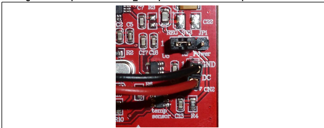
Figure 5. Jumper JP1 in “REG_3V3” position and external power connection
