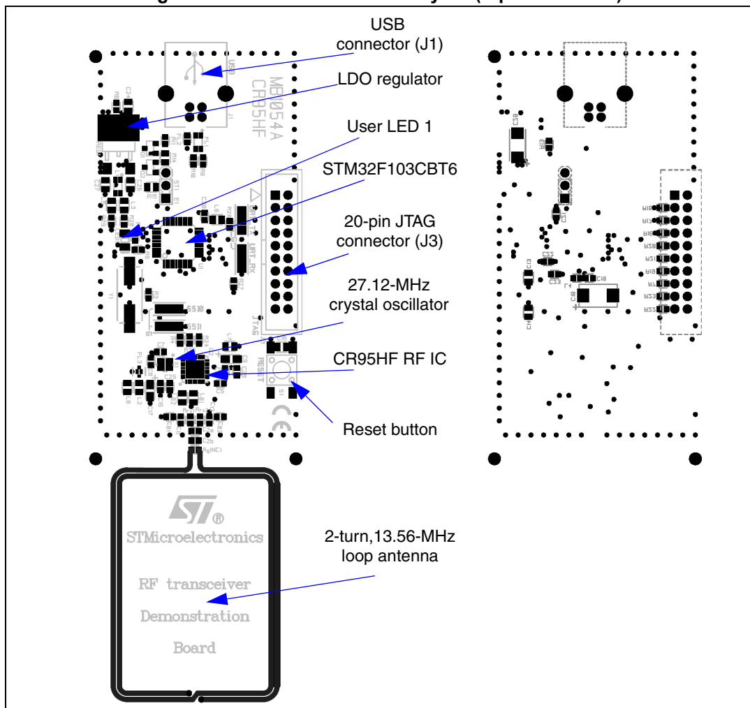
Figure 8. RF transceiver board layout (top and bottom)
