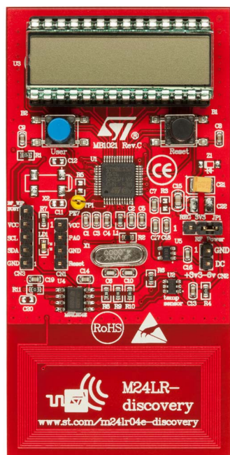
M24LR board
