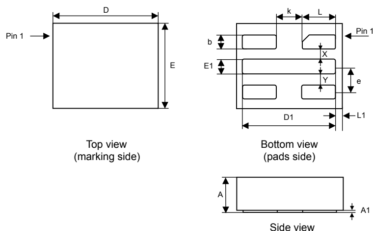
Figure 13. UFDFPN5 - Outline
