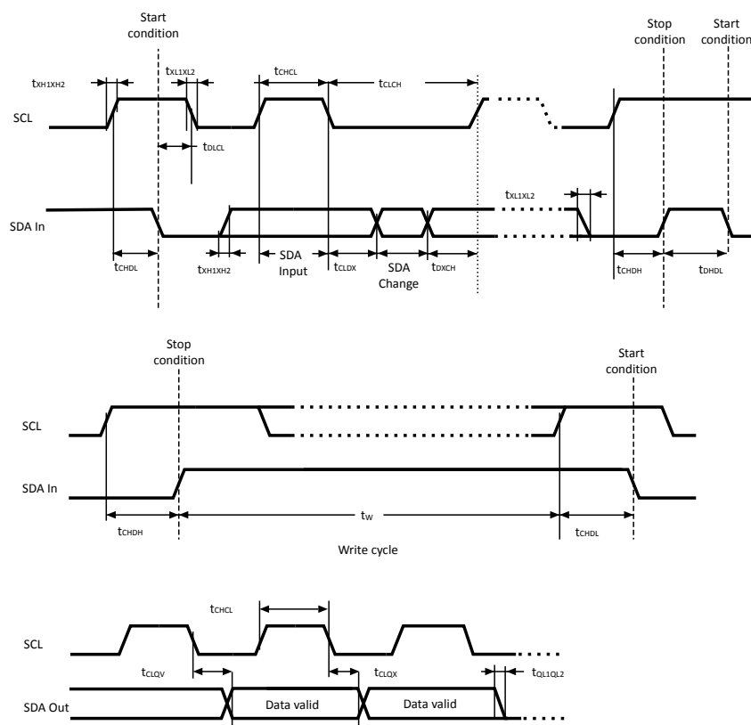
Figure 12. AC waveforms
