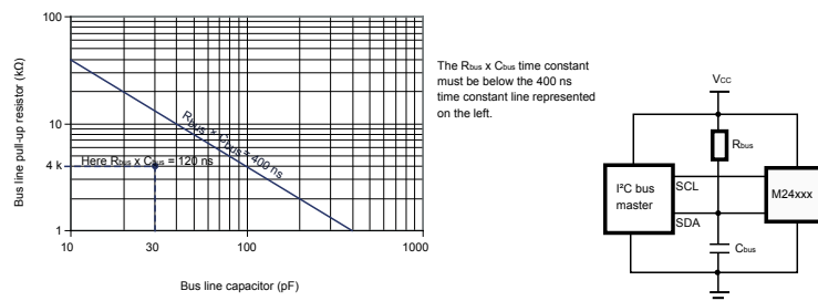
Figure 11. Maximum R_{\text{BUS}} value versus bus parasitic capacitance ( C_{\text{BUS}} ) for an I 2 C bus at maximum frequency f_C = 400 kHz
