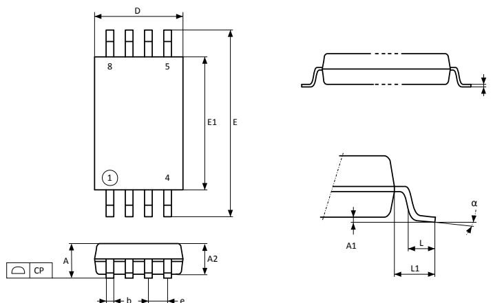
Figure 17. TSSOP8 – Outline
