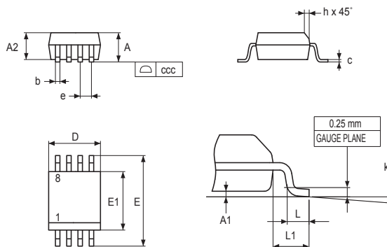
Figure 19. SO8N – Outline
