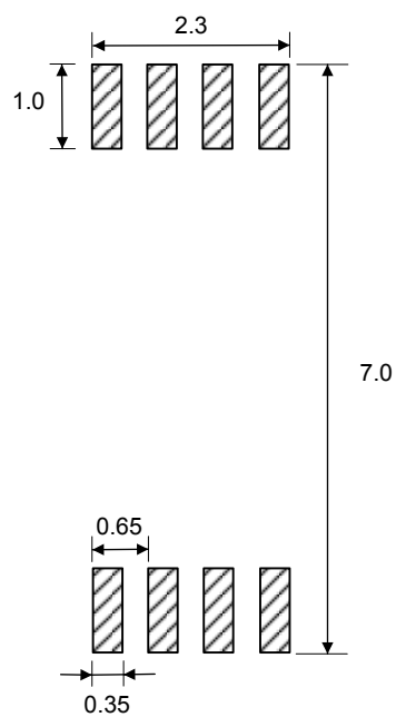
Figure 18. TSSOP8 – Recommended footprint
