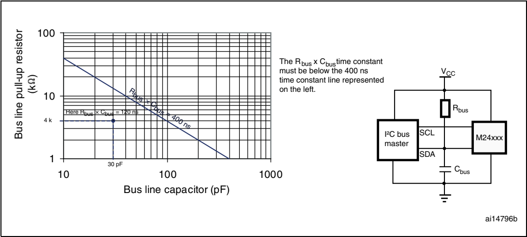
Figure 9. Maximum R_{bus} value versus bus parasitic capacitance ( C_{bus} ) for an I 2 C bus at maximum frequency f_C = 400\text{ kHz}
