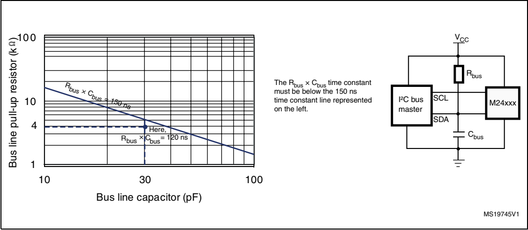
Figure 10. Maximum R_{bus} value versus bus parasitic capacitance ( C_{bus} ) for an I 2 C bus at maximum frequency f_C = 1\text{ MHz}
