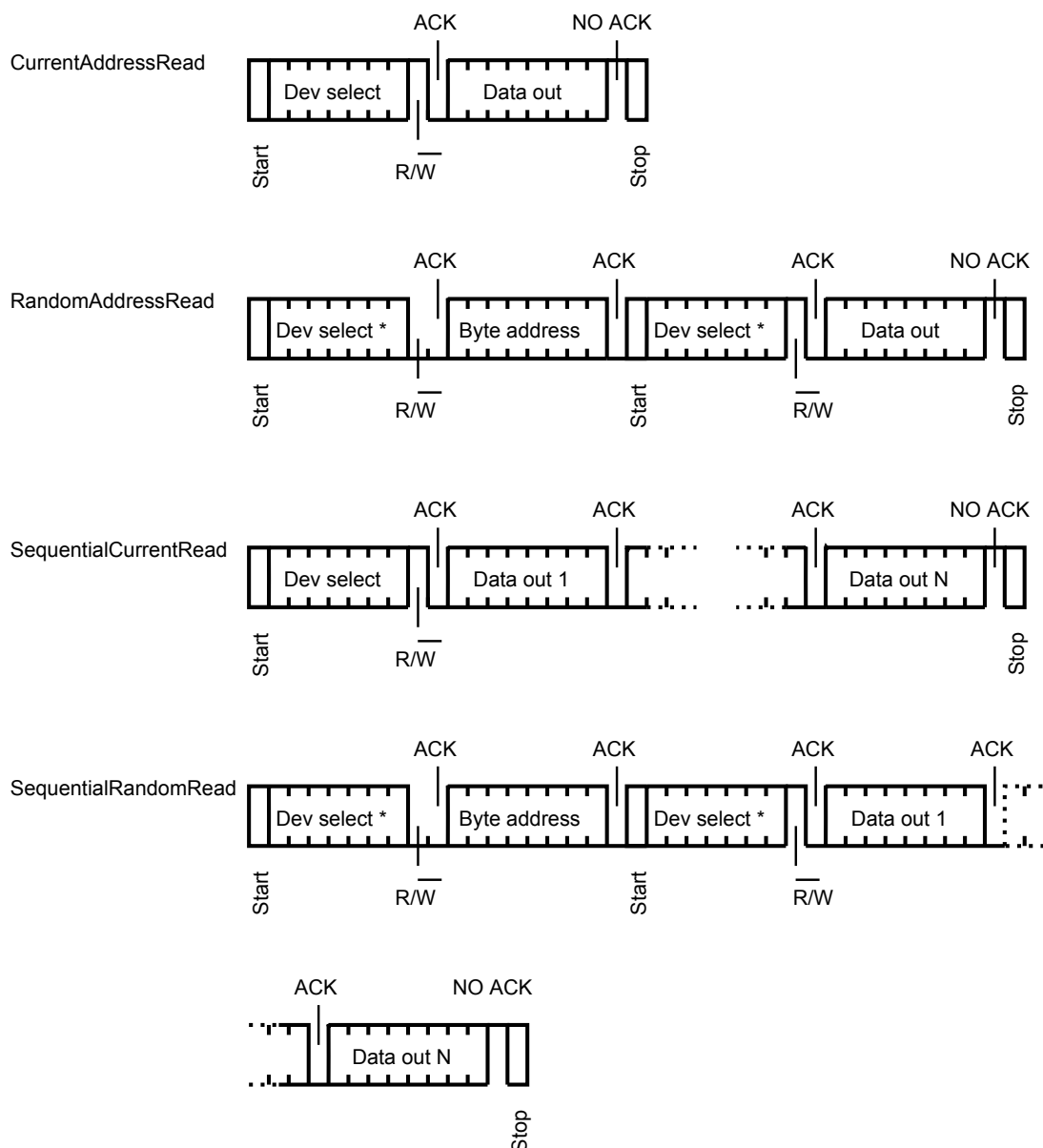
Figure 8. Read mode sequences
