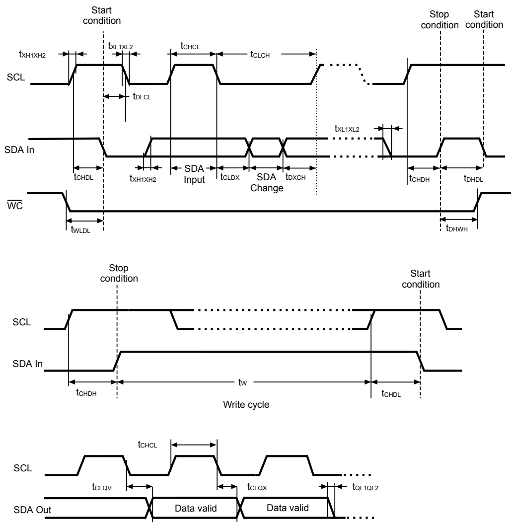
Figure 12. AC waveforms
