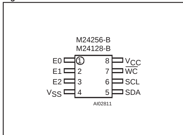
Figure 2B. SO8 and TSSOP8 Connections
