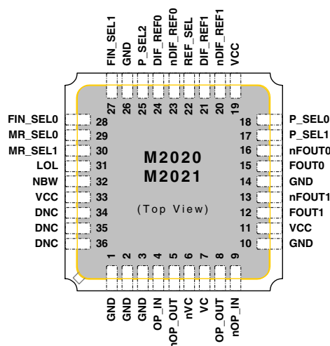
Figure 1: Pin Assignment
