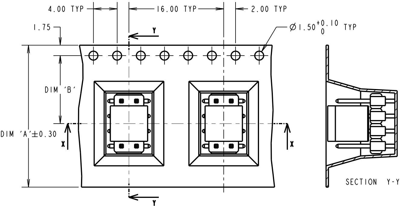
TAPE DETAILS FOR 02, 03 & 04 WAYS
