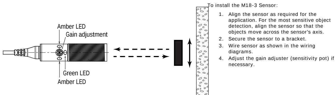
Figure 1. M18-3 Features and Installation
