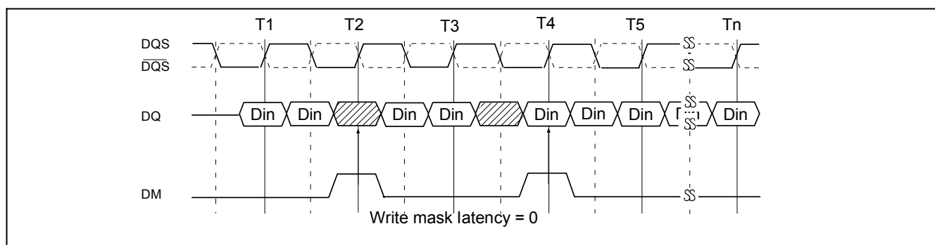
Data Mask Timing
