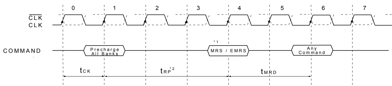
Mode Register
