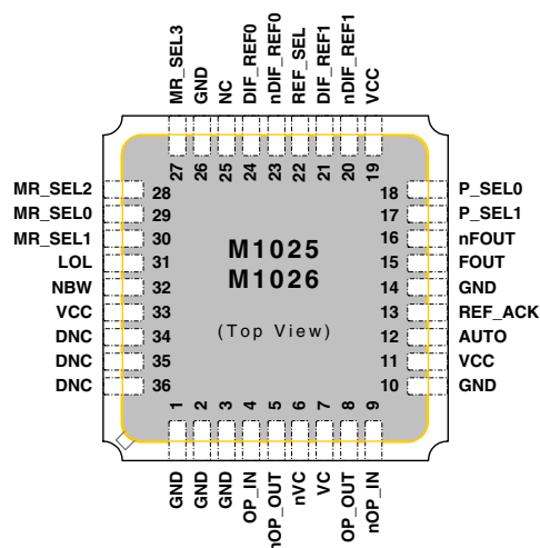
Figure 1: Pin Assignment
