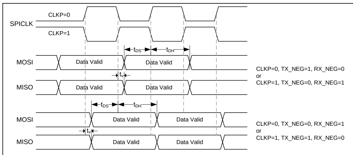
Figure 7.6-2 SPI Slave Mode Timing
