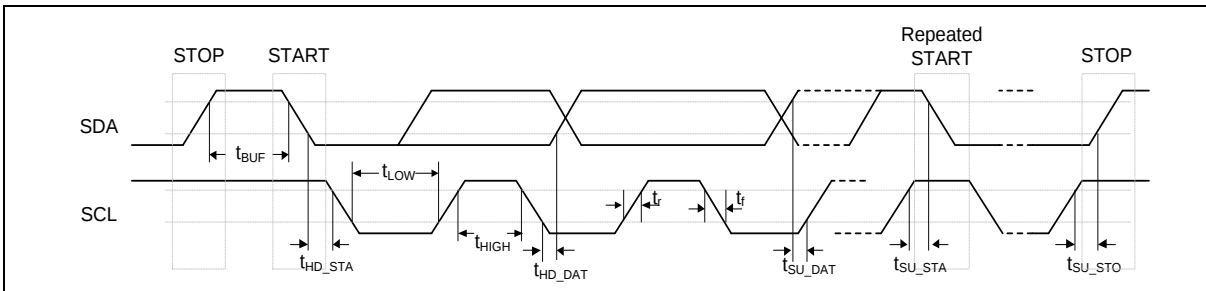
Figure 6.21-1 I 2 C Bus Timing
