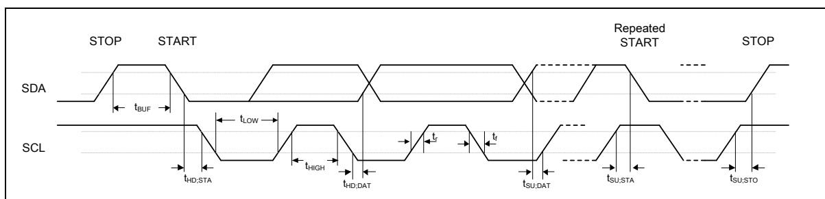
Figure 8-4 I 2 C Timing Diagram
