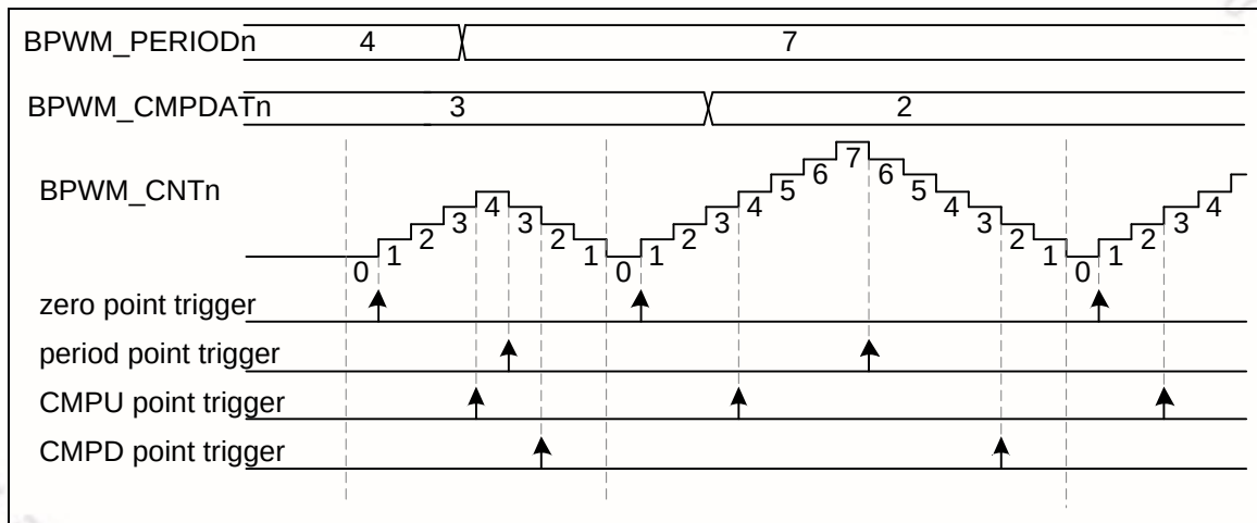
Figure 6-77 BPWM Trigger ADC in Up-Down Counter Type Timing Waveform
