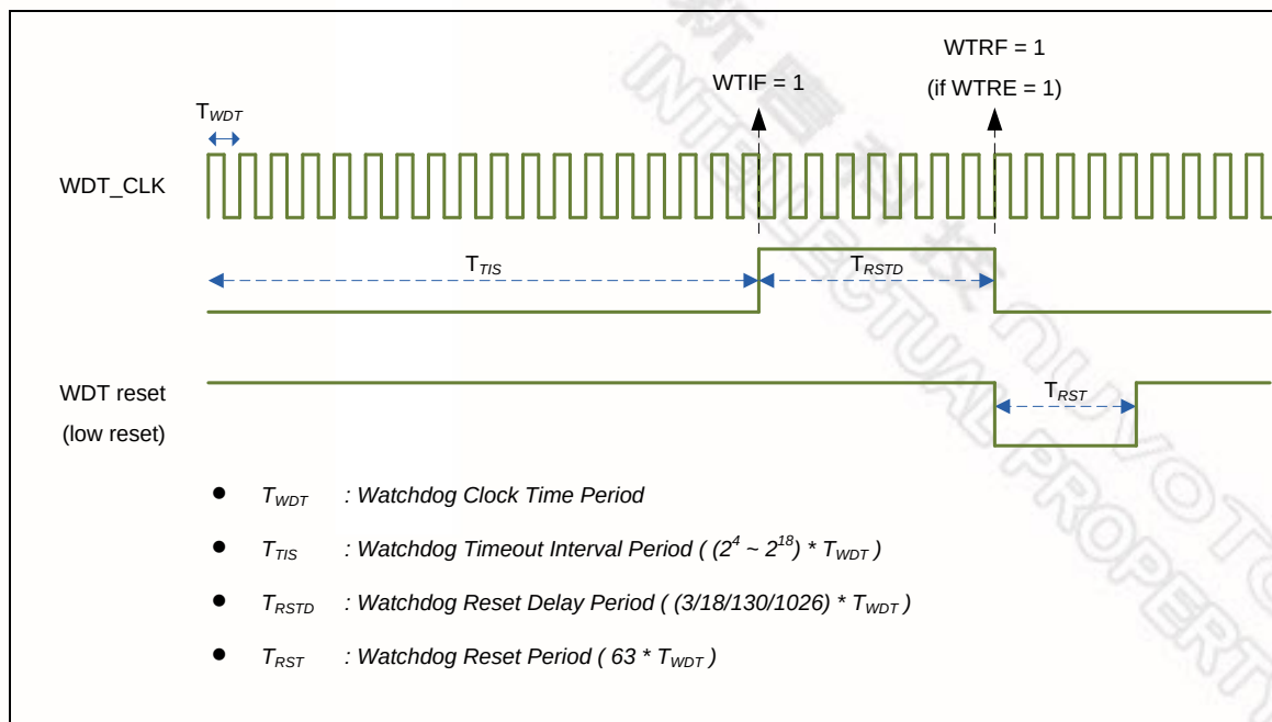
Figure 6-82 Watchdog Timer Time-out Interval and Reset Period Timing
