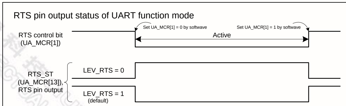
Figure 6-93 UART RTS Flow with Software Control
