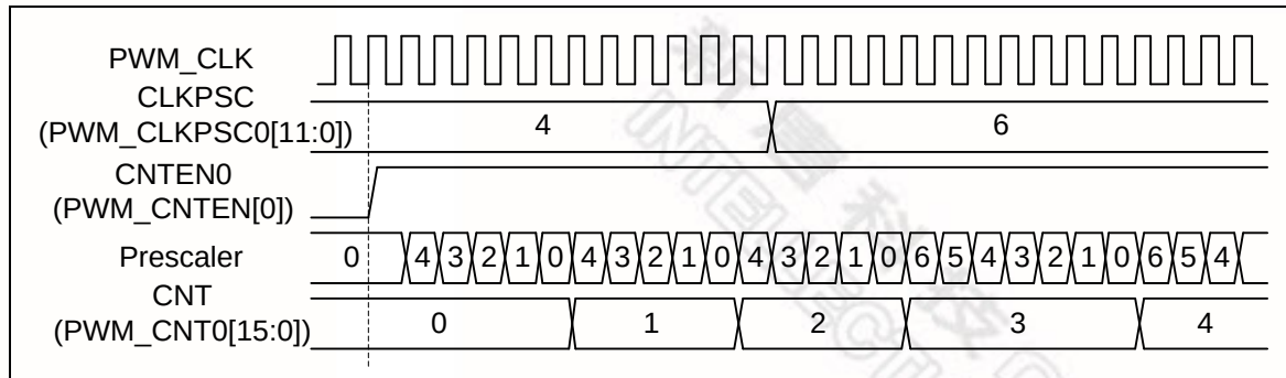
Figure 6-28 PWM_CH0 CLKPSC waveform
