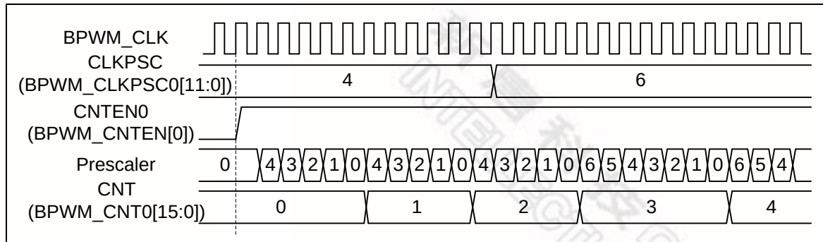
Figure 6-61 BPWM_CH0 CLKPSC waveform
