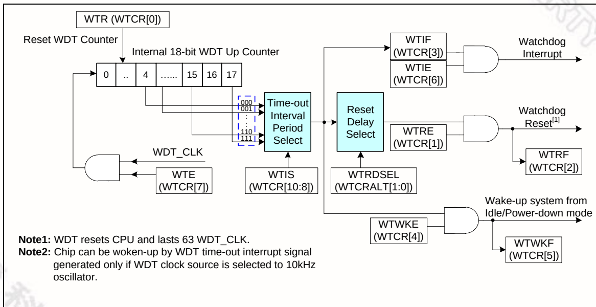
Figure 6-81 Watchdog Timer Block Diagram
