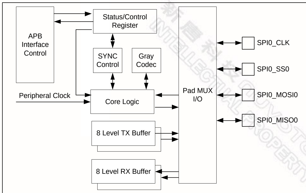
Figure 6-124 SPI Block Diagram
