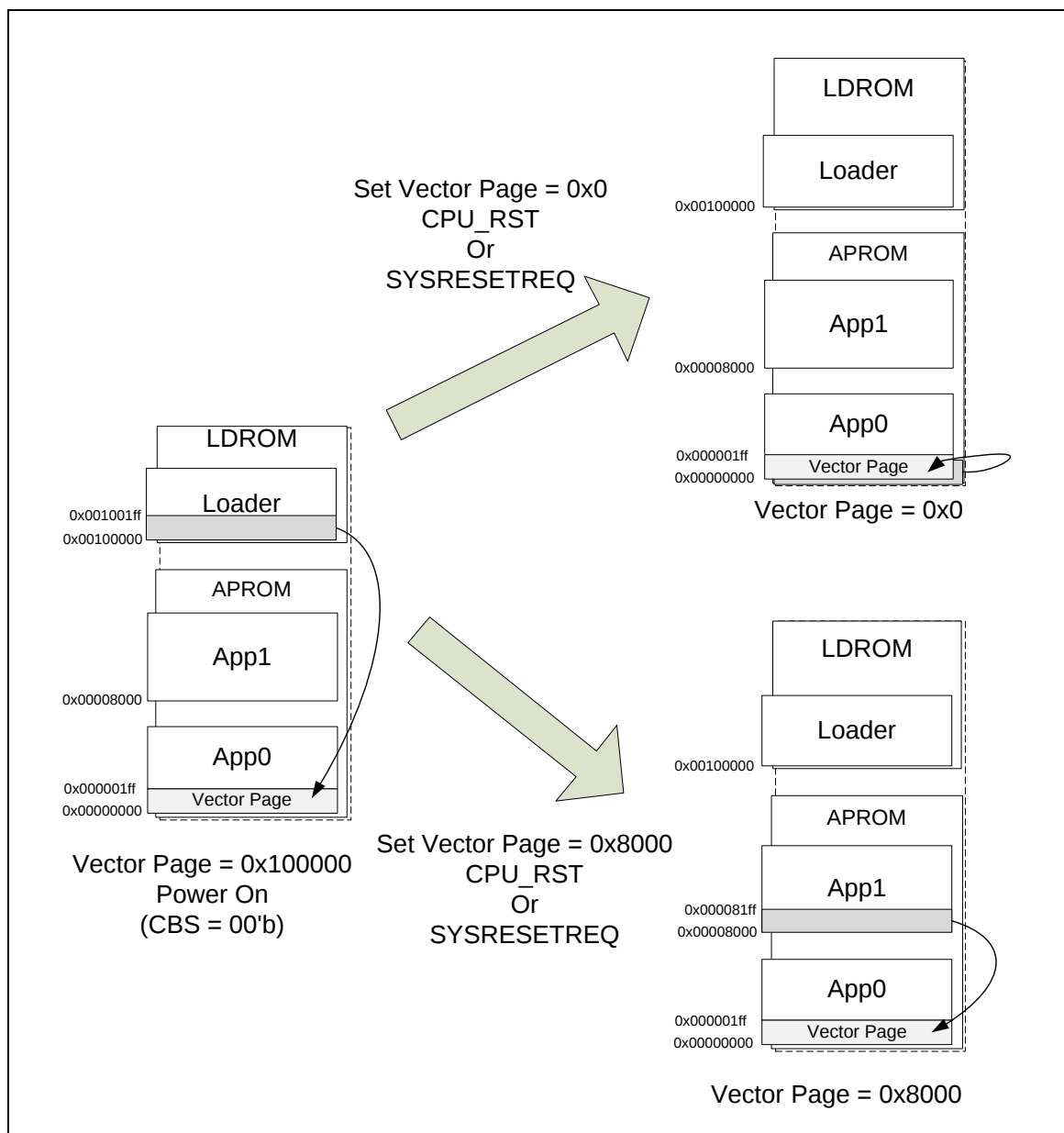
Figure 6-18 Multi-booting by Vector Page Remapping
