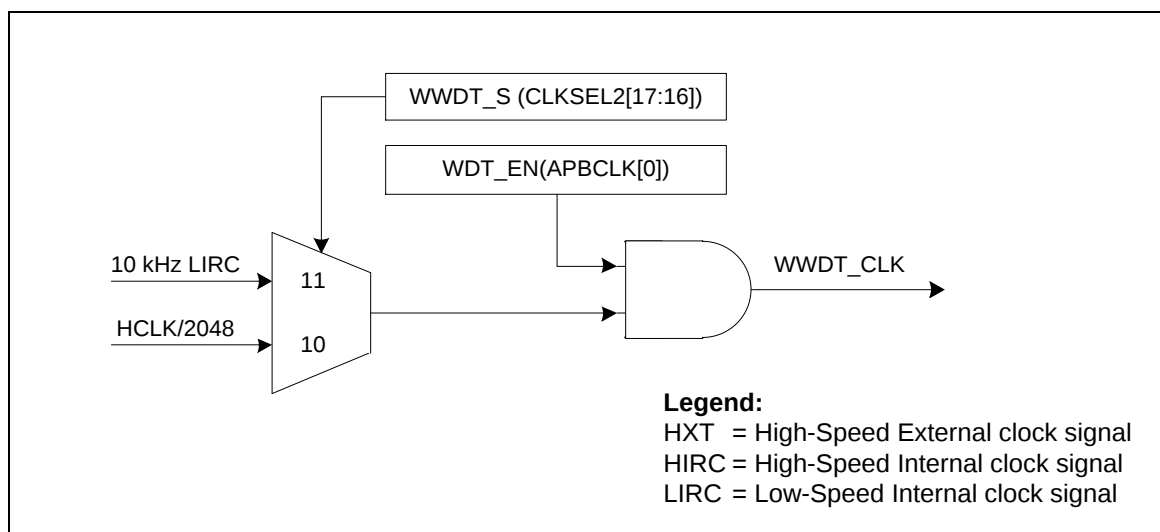
Figure 6-57 Window Watchdog Timer Clock Control
