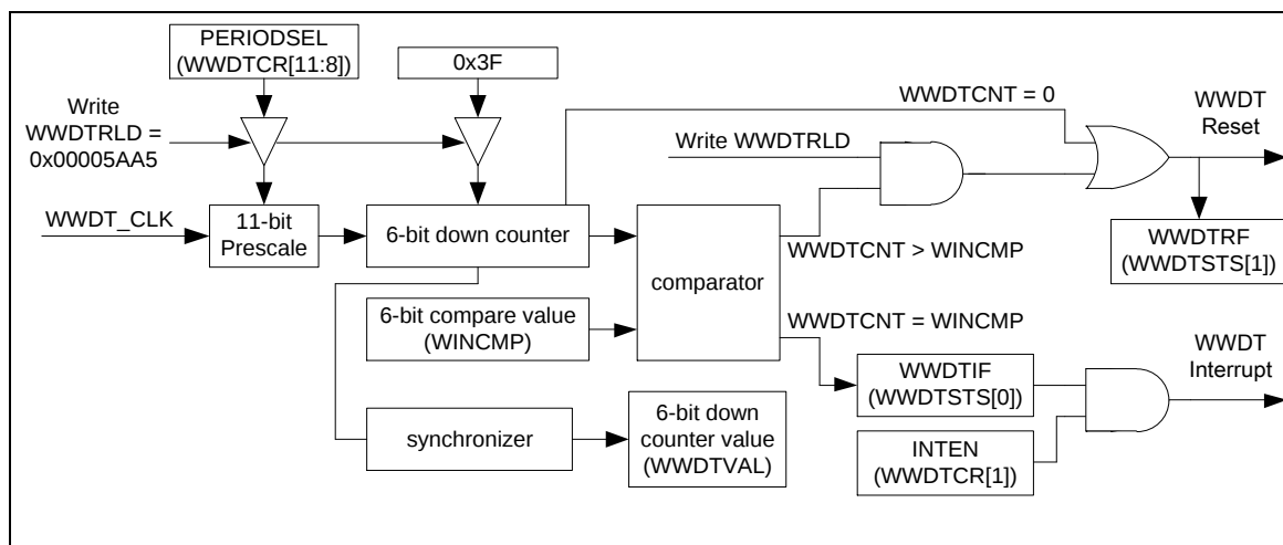
Figure 6-58 Window Watchdog Timer Block Diagram
