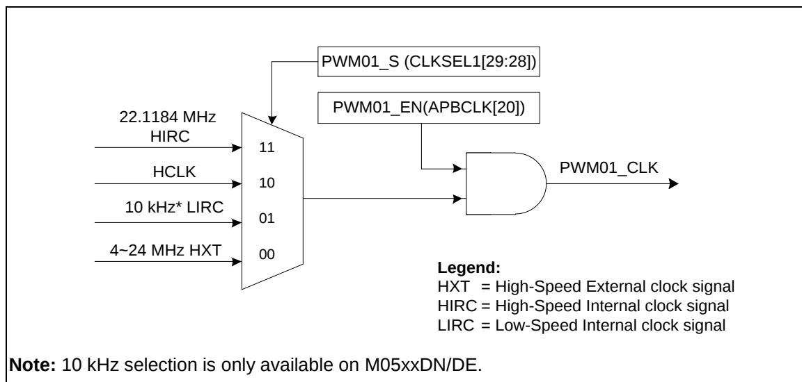
Figure 6-32 PWM Generator 0 Clock Source Control
