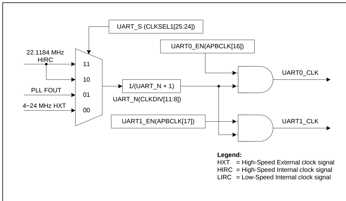
Figure 6-60 UART Controller Clock Control
