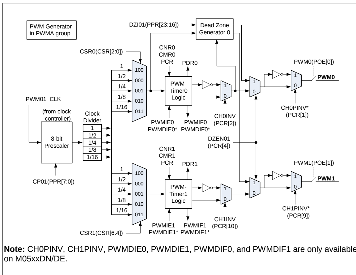
Figure 6-33 PWM Generator 0 Architecture Diagram
