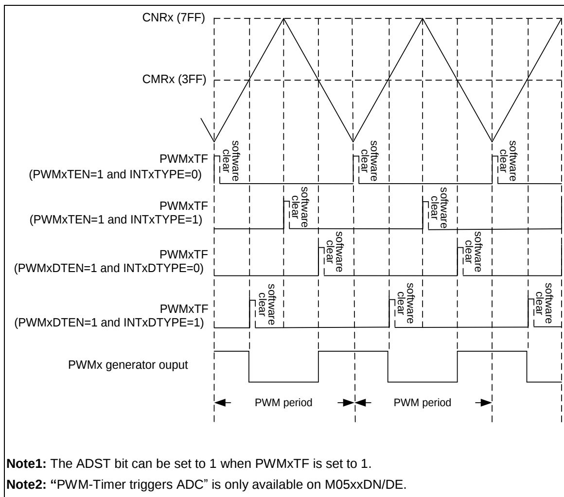
Figure 6-48 PWM Trigger ADC Flag (PWMxTF) in Center-aligned Type Timing Waveform
