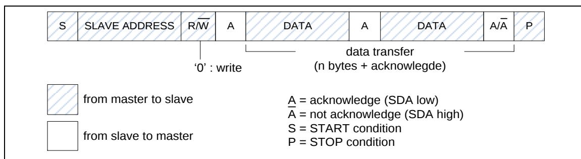
Figure 6-77 Master Transmits Data to Slave
