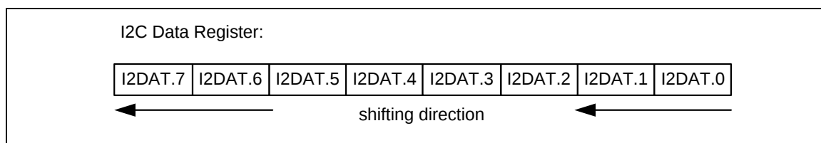
Figure 6-79 I 2 C Data Shifting Direction
