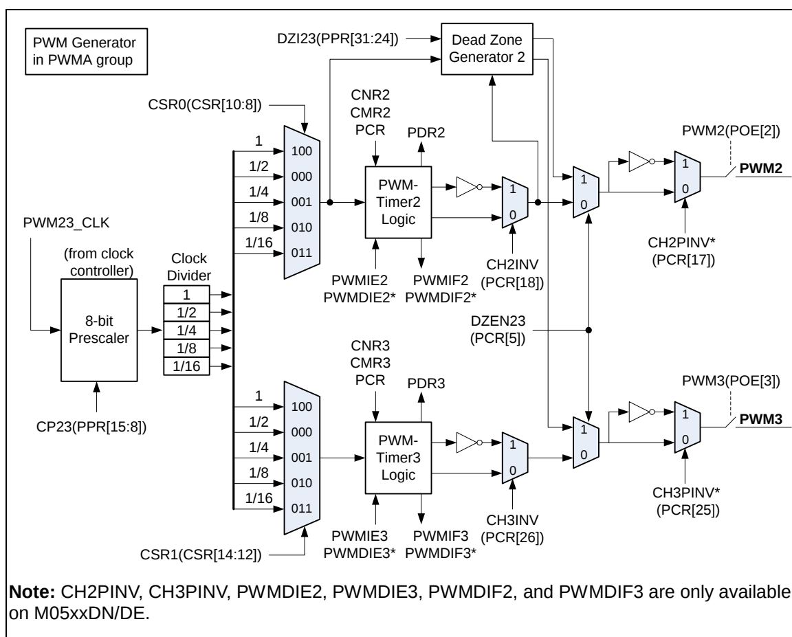
Figure 6-35 PWM Generator 2 Architecture Diagram
