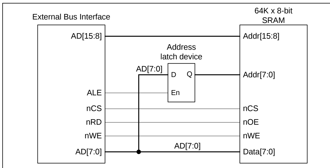
Figure 6-21 Connection of 8-bit EBI Data Width with 8-bit Device
