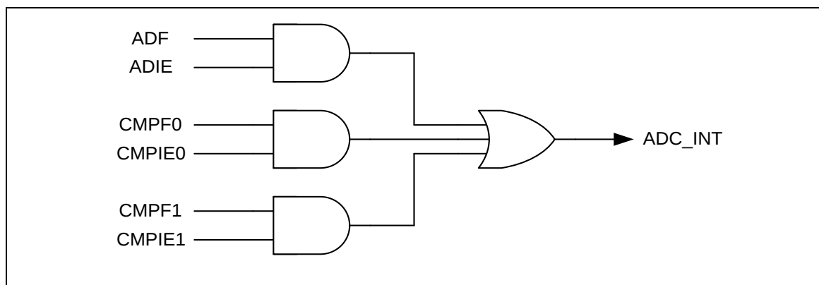
Figure 6-107 A/D Controller Interrupt
