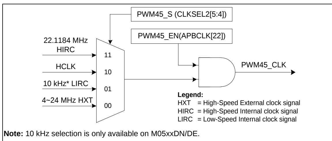
Figure 6-36 PWM Generator 4 Clock Source Control
