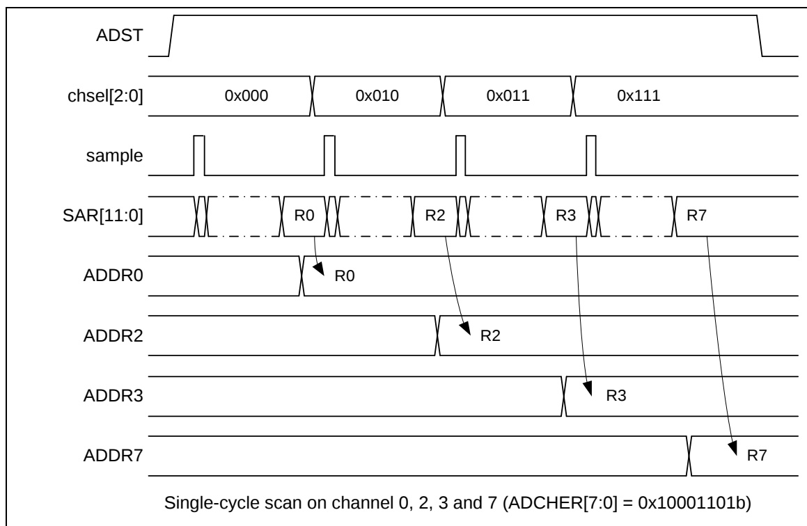
Figure 6-103 Single-Cycle Scan Mode on Enabled Channels Timing Diagram
