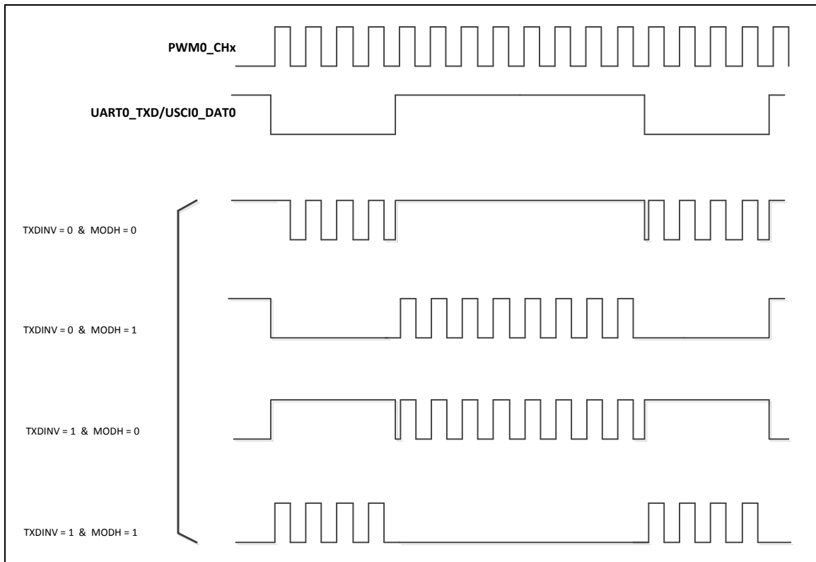
Figure 6.2-11 UART0_TXD/USC10_DAT0 Modulated with PWM Channel
