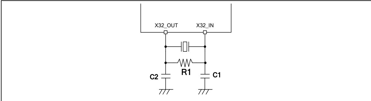
Figure 8.4-4 Typical 32.768 kHz Crystal Application Circuit
