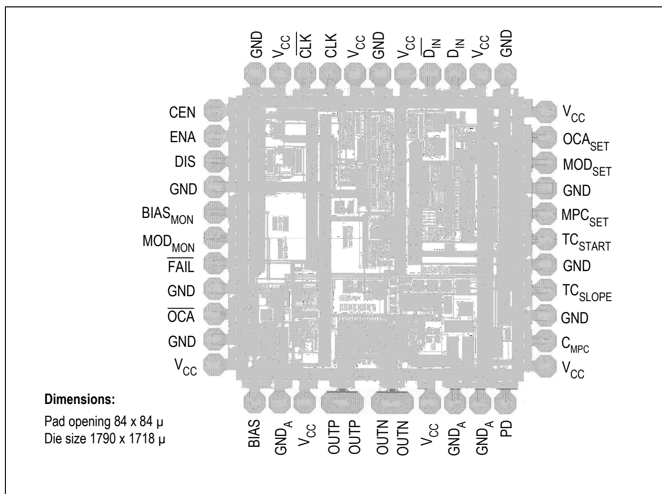
Figure 4-1. Bare Die Information
