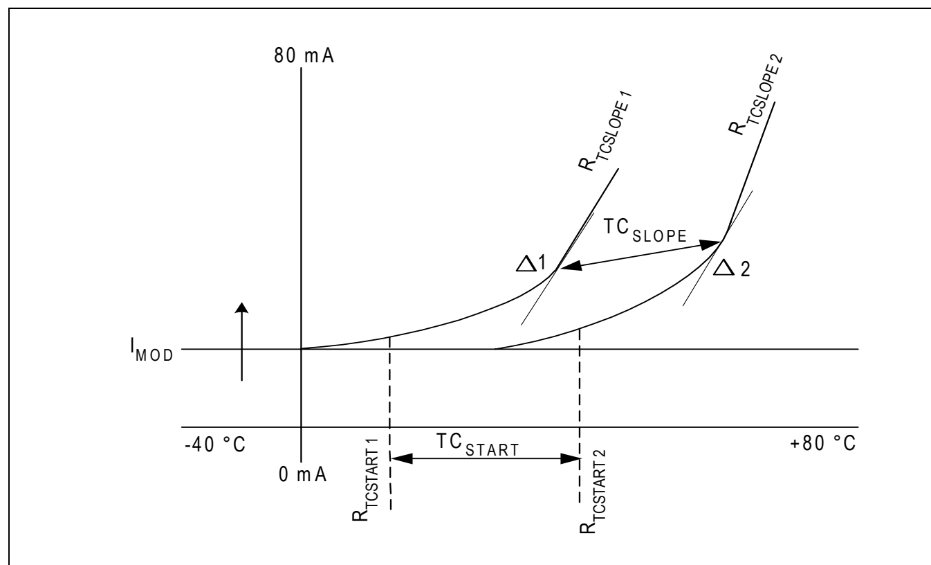
Figure 3-6. Temperature Compensation
