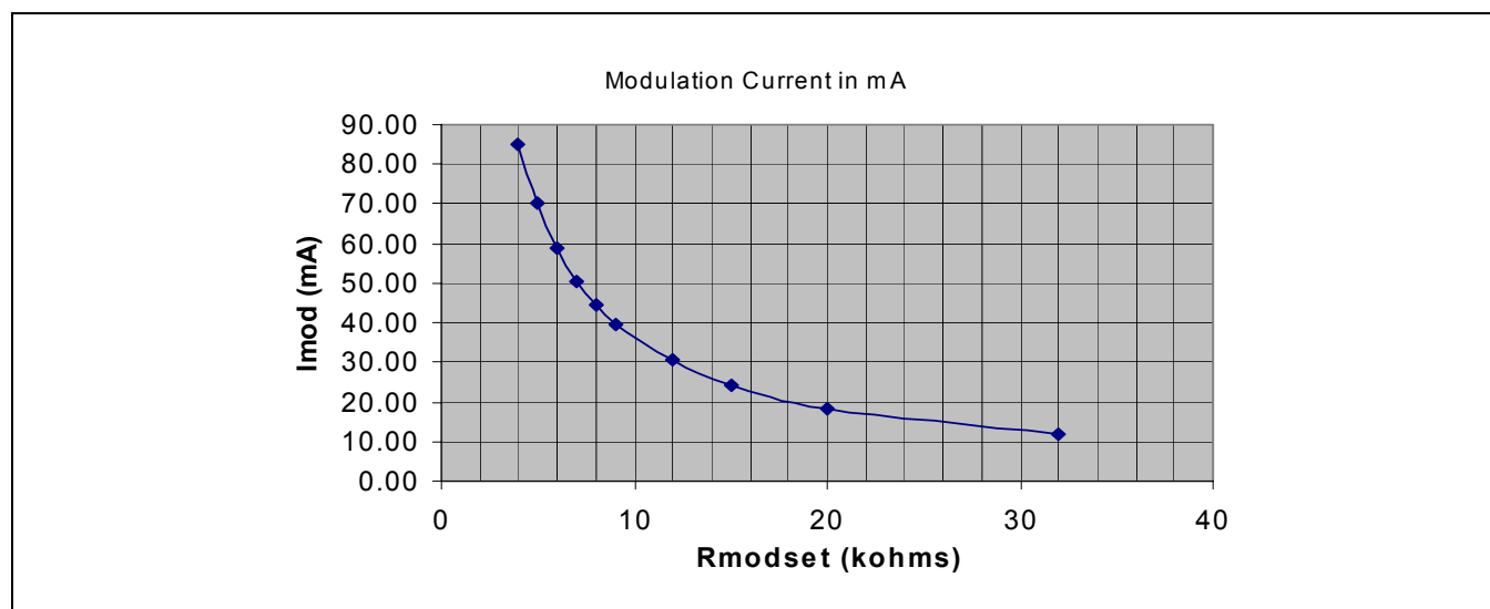
Figure 3-2. Modulation Current vs. R_{MODSET}
