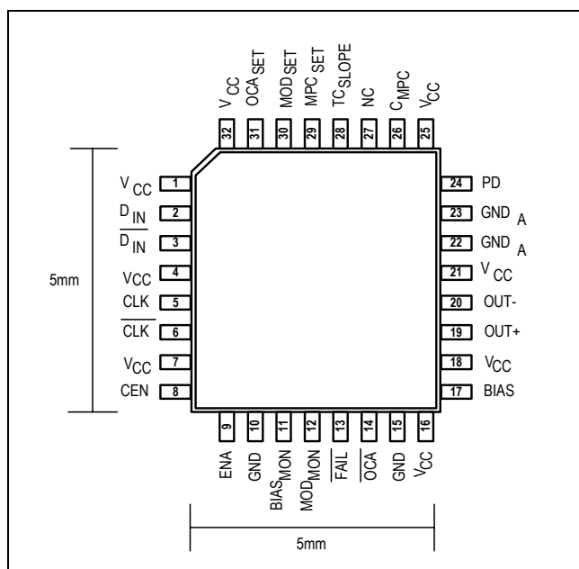
TQFP32 Top View
