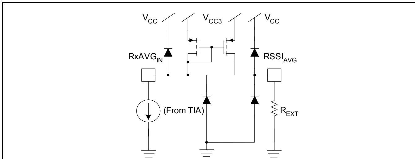
Figure 3-11. RSSI_{AVG} Output
