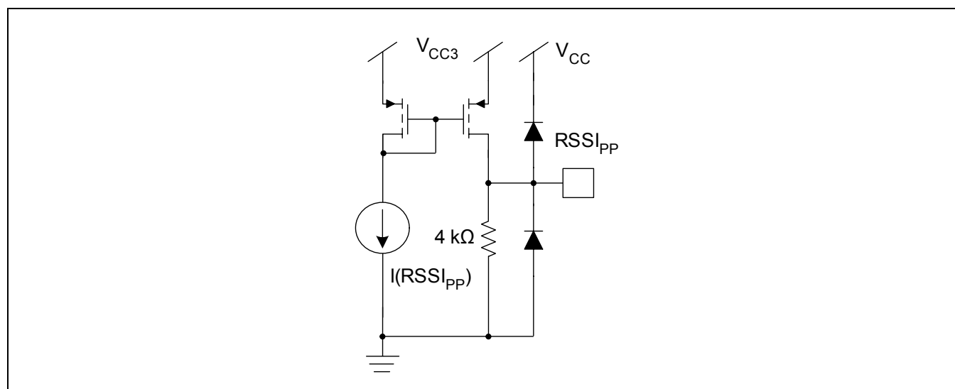
Figure 3-6. RSSI PP Output
