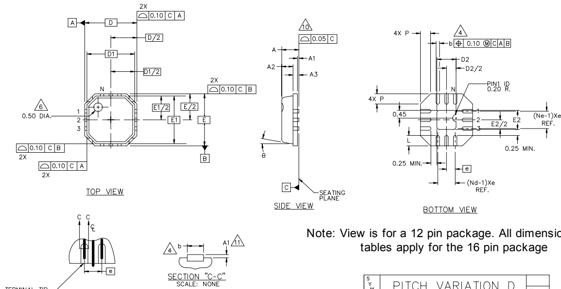
Figure 5-1. Package Information
