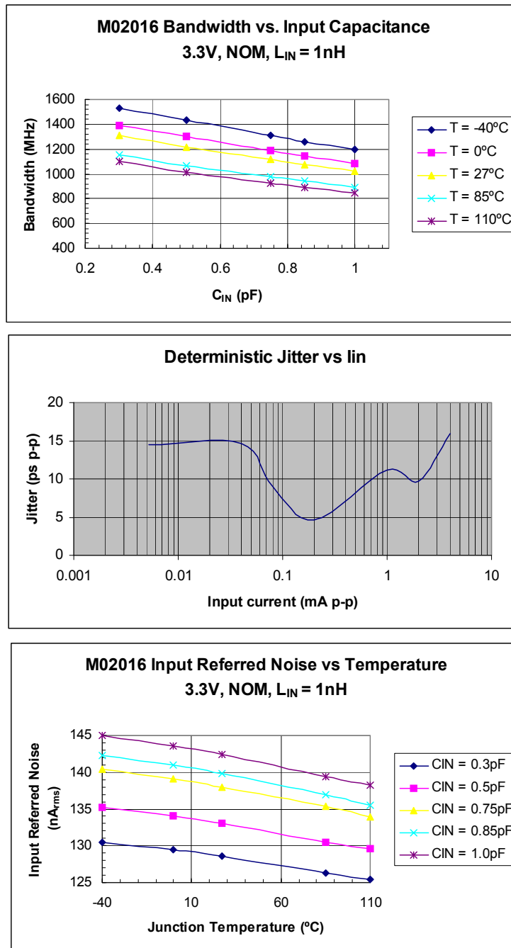
Figure 1-2. Typical Performance Diagrams 2 of 3
