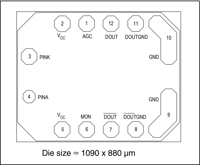
Pad Configuration
