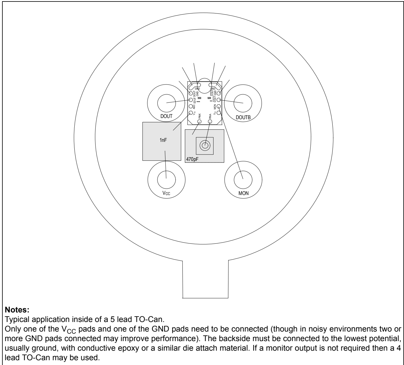
Figure 4-2. Typical Layout Diagram
