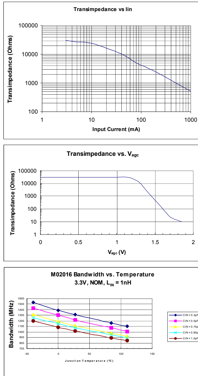
Figure 1-1. Typical Performance Diagrams 1 of 3
