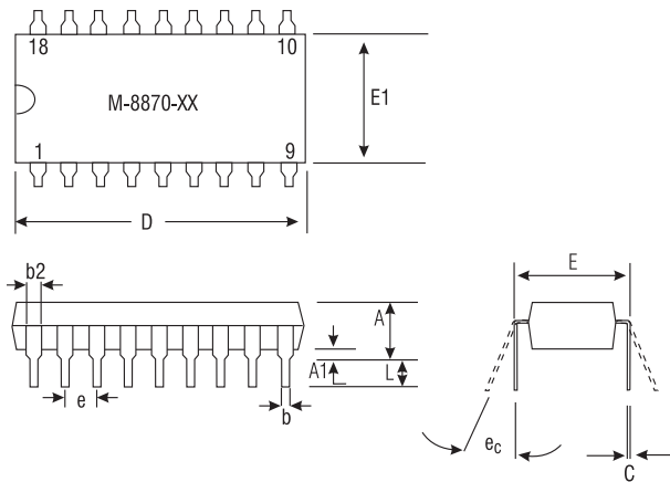
Figure 9 Mechanical Dimensions
