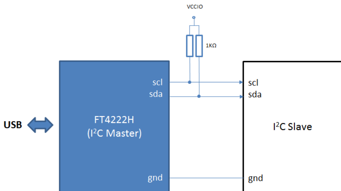
Figure 1.3 Mode 0: FT4222H works as I²C Master
