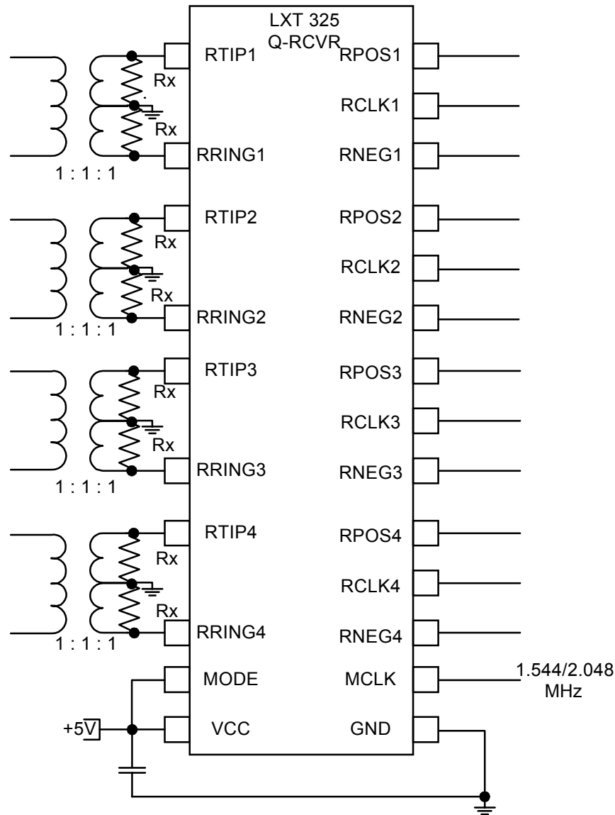
Figure 3: Typical DSX-1/E1 Receiver Application
