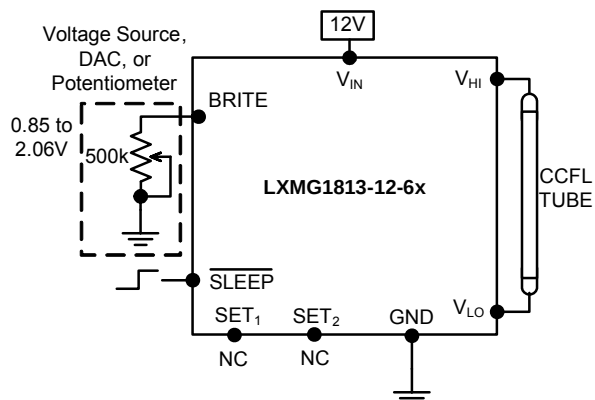
Figure 1 – Brightness Control
