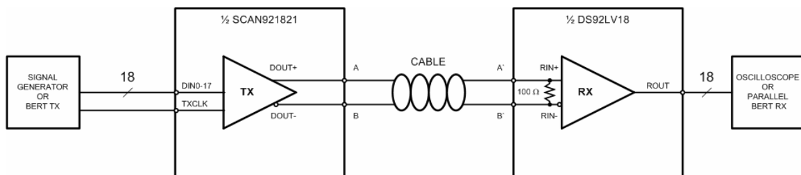
Figure 5. Test Setup for the SerDes Chipset Cable Drive Application
