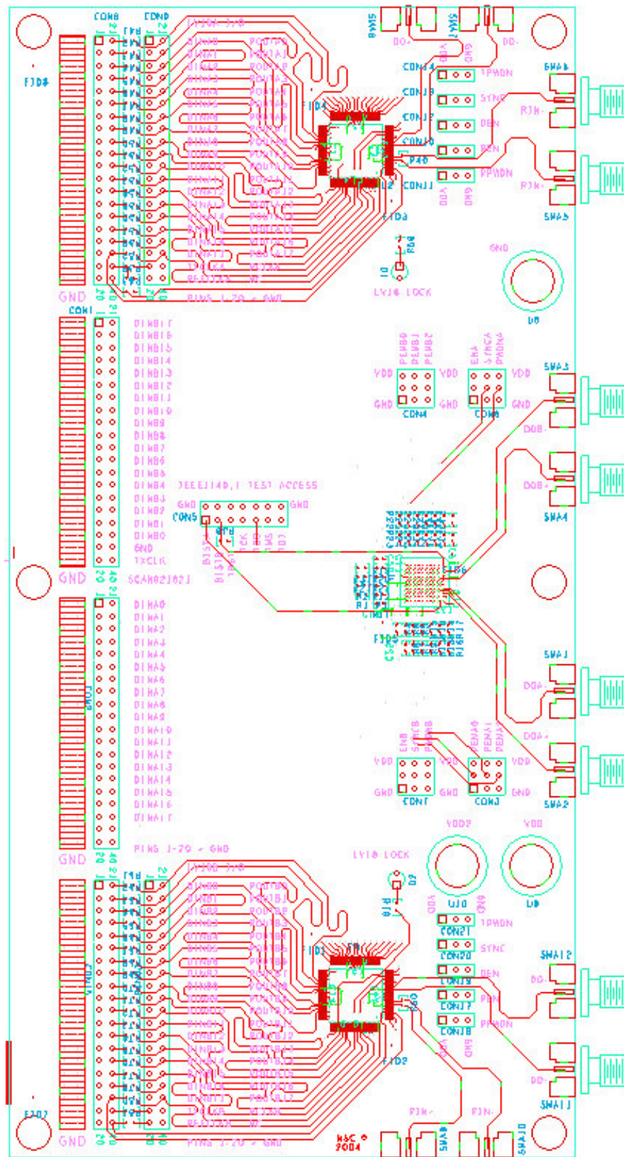
Figure 1: LVDS-18B-EVK Evaluation Board Top View
