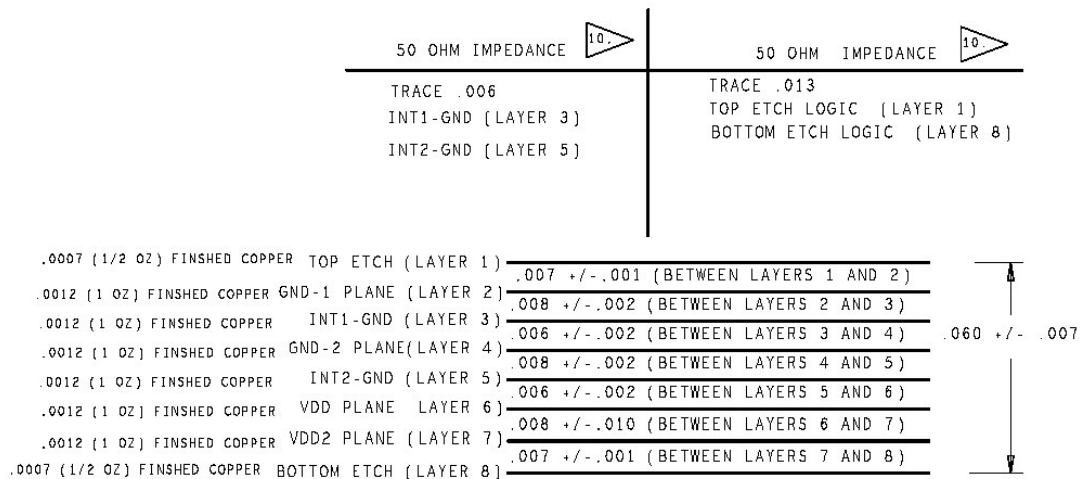
Figure 2: Board Stack up Detail
