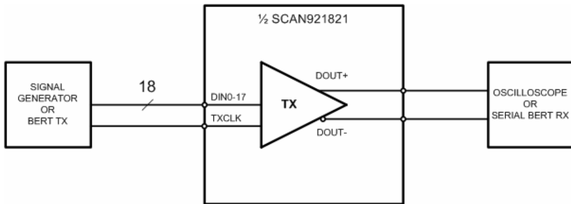
Figure 3. Test Setup for the SCAN921821 Only
