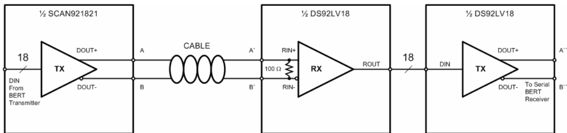
Figure 6. Test Setup for the SerDes Chipset Cable Drive Application
