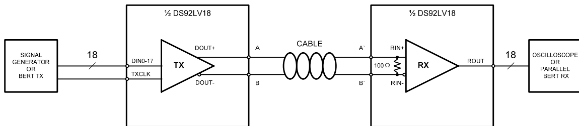
Figure 4. Test Setup for the SerDes Chipset Cable Drive Application
