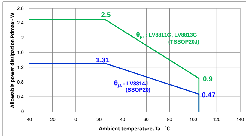
Figure 6. Power Dissipation vs Ambient Temperature Characteristic
