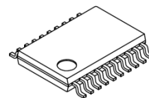
LV8811G, LV8813G : 20-pin TSSOP with exposed pad CASE 948AZ
