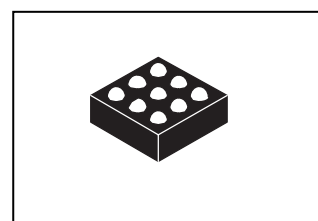
WLP9, 1.31x1.31, 0.4mm pitch (1.31mm x 1.31mm, Amax=0.625 mm)
