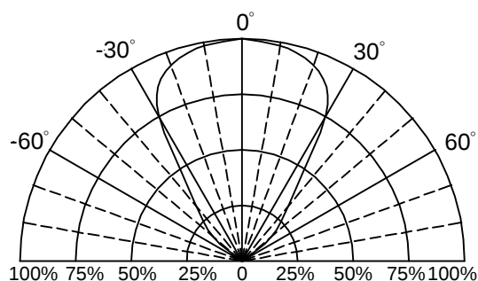
Fig.6 Directivity Radiation
