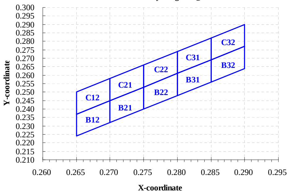
C. I. E. 1931 Chromaticity Diagram @5mA
