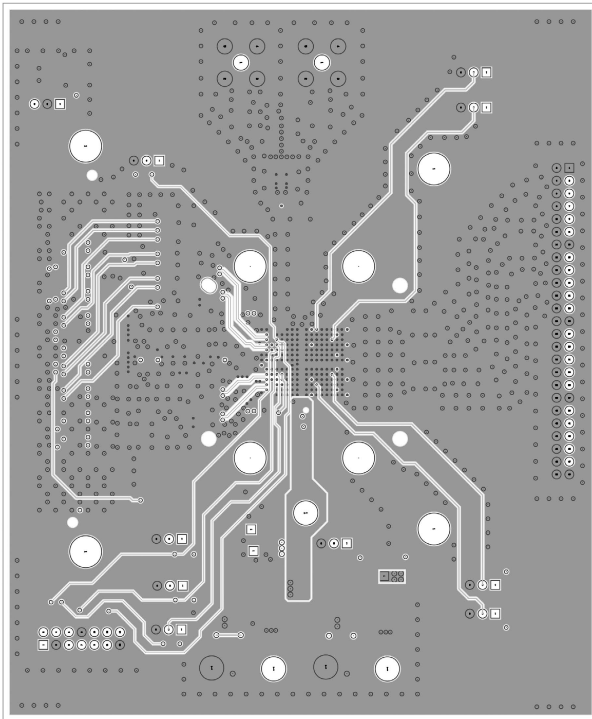
Figure 9. Layer 3
