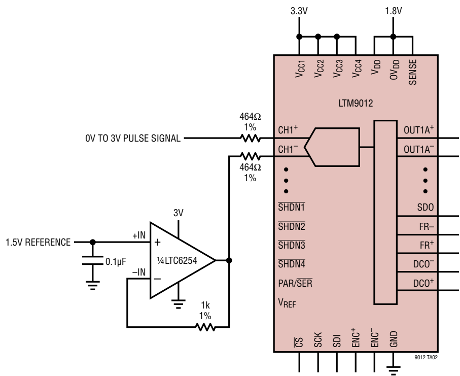
Single-Ended Drive with Unity Gain Example
