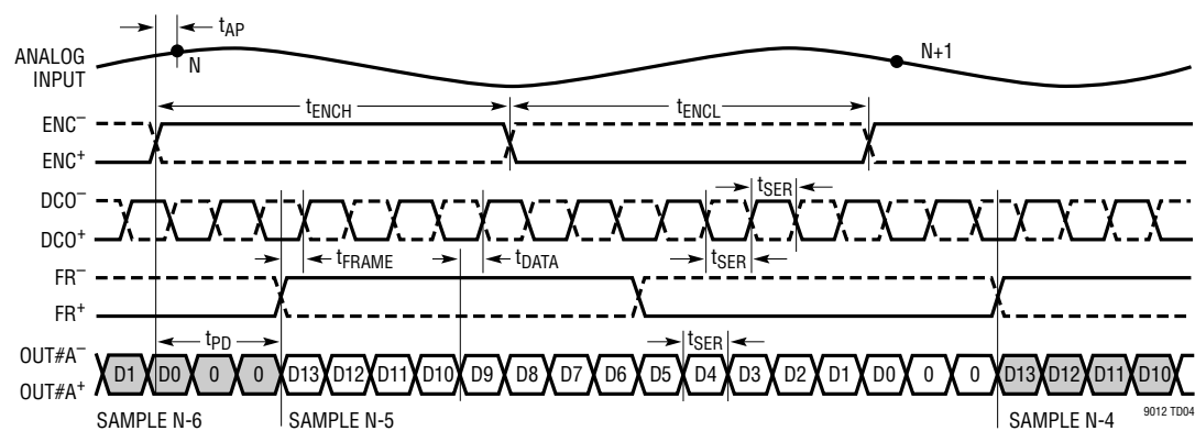
1-Lane Output Mode, 16-Bit Serialization
