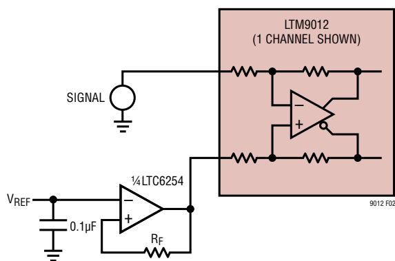
Figure 2. Single-Ended Operation
