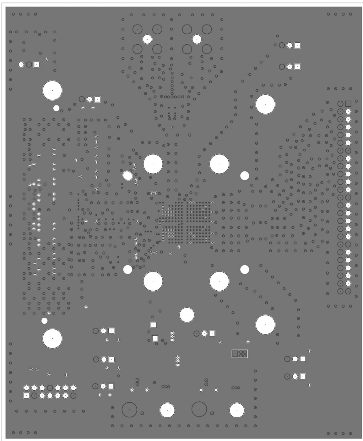
Figure 8. Layer 2
