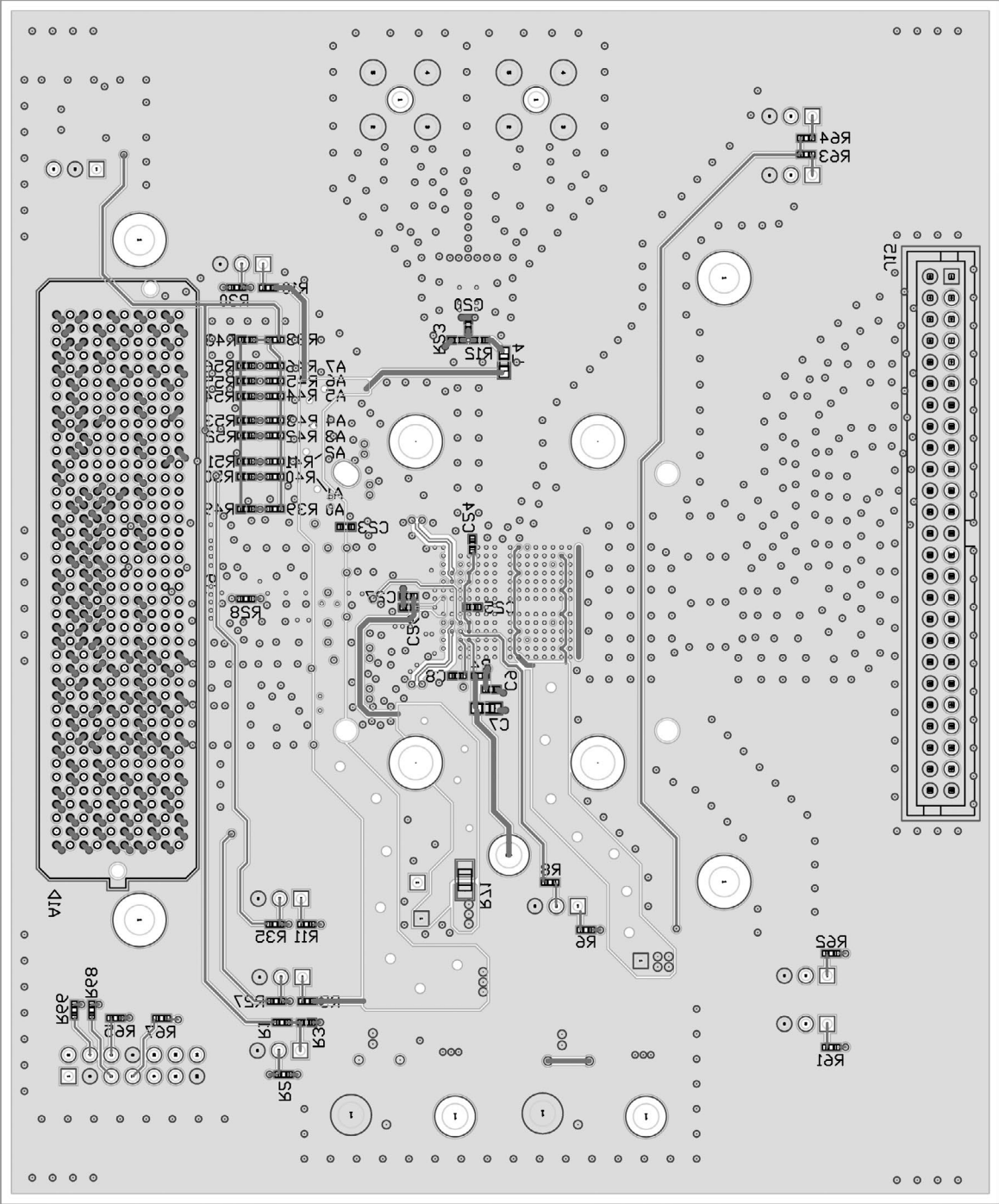
Figure 10. Back Side
