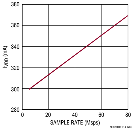
LTM9009-14: I_{VDD} vs Sample Rate, 5MHz Sine Wave Input, -1dBFS
