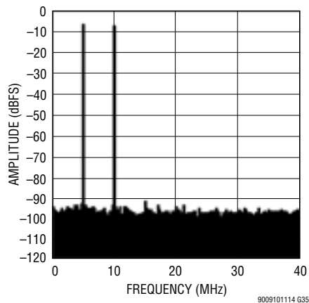
LTM9009-14: 8k Point 2-Tone FFT, f_{IN} = 70\text{MHz} , 75MHz, -7\text{dBFS} per Tone, 80Mps
