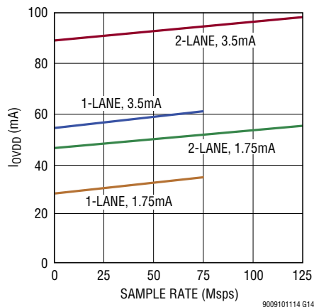
I_{OVD} vs Sample Rate, 5MHz Sine Wave Input, -1dBFS
