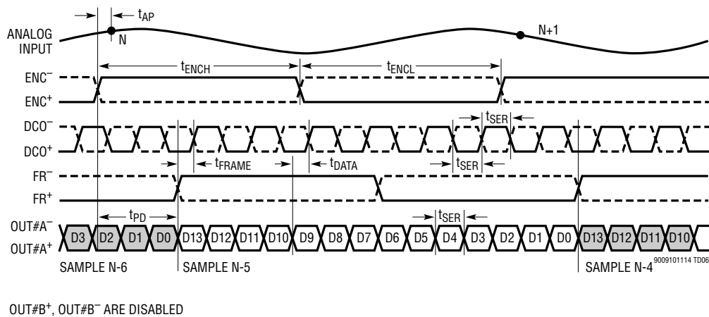
1-Lane Output Mode, 14-Bit Serialization
