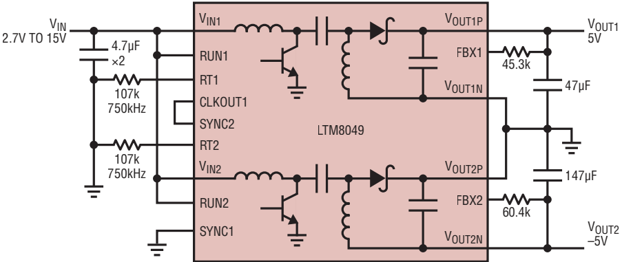
±5V Converter
