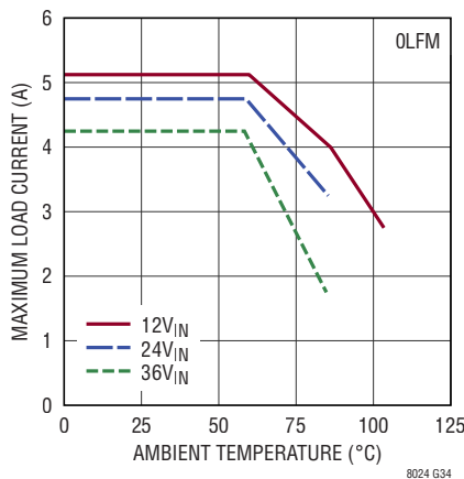
Derating, V_{OUT} = 8\text{V} , BIAS = 5V, DC1868A Demo Board Channel 2 Off
