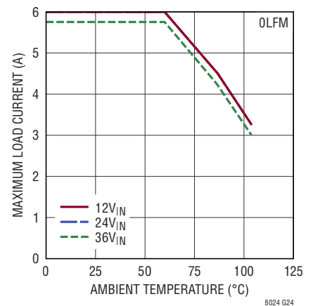
Derating, V_{OUT} = 2.5\text{V} , BIAS = 5V, DC1868A Demo Board Both Channels at Same Load
