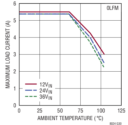
Derating, V_{OUT} = 8\text{V} , BIAS = 5V, DC1868A Demo Board Both Channels at Same Load
