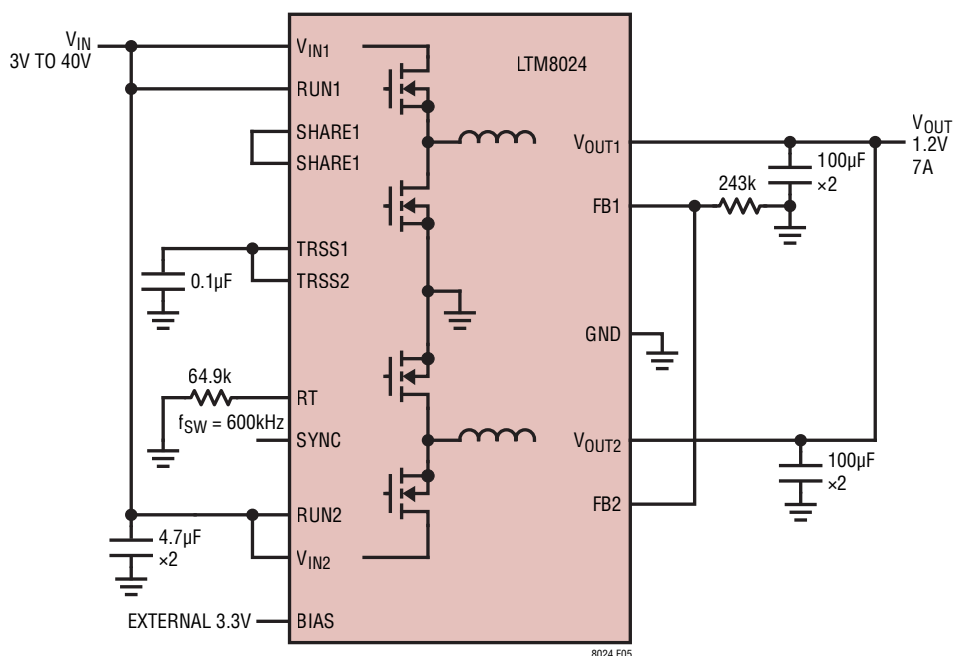
Figure 5. Parallel Two Channels to Produce 1.2V/7A from 3V to 40V IN . BIAS is Tied to External 3.3V
