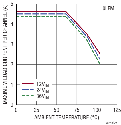
Derating, V_{OUT} = 1.8\text{V} , BIAS = 5V, DC1868A Demo Board Channel 2 Off
