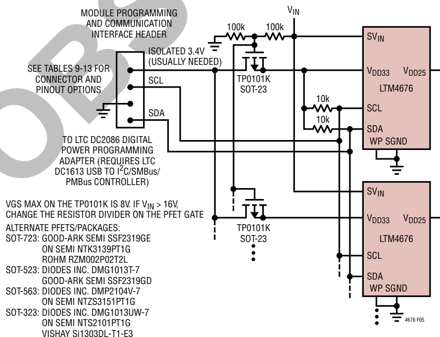
Figure 5. Circuit Suitable for Programming EEPROM/NVM of LTM4676 and Other LTC PSM Modules/ICs in Vast Systems, Even When V_{IN} Power Is Absent, 0^{\circ}\text{C} < T_J < 85^{\circ}\text{C}
