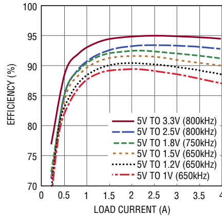
Efficiency vs Load Current at 5\text{V}_{\text{IN}} , CCM Mode
