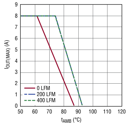
Figure 24. 20V IN , 5V OUT 1.2MHz, with Heat Sink
