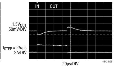
5\text{V}_{\text{IN}} to 1.5\text{V}_{\text{OUT}} Transient Response
