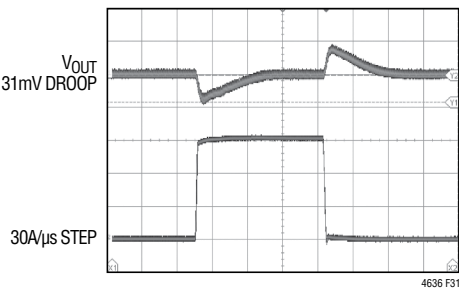
INTERNAL COMPENSATION C OUT = 8X 470μF 6V TPD POS CAP, 16 × 100μF CERAMIC FURTHER OPTIMIZATION CAN BE UTILIZED WITH EXTERNAL COMP
