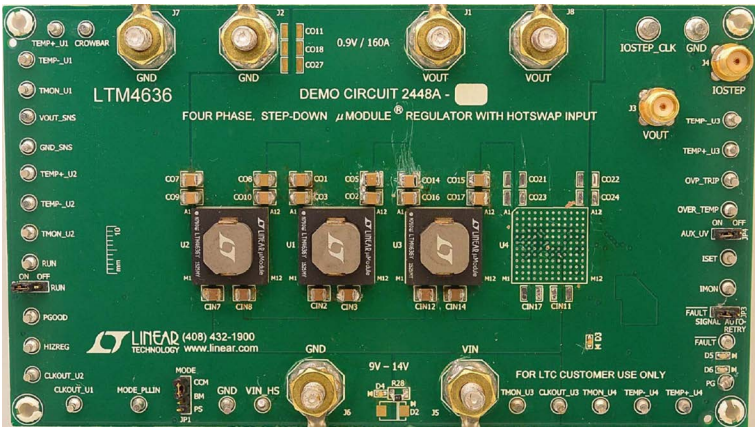
Figure 23. Demo Board
