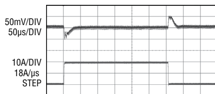
1V Transient Response
