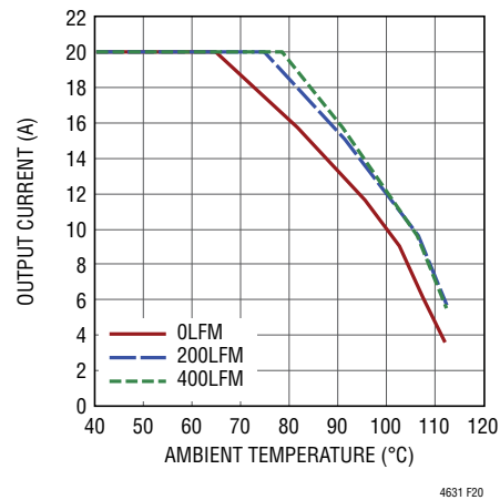
Figure 20. 5V to 1.5V Derating Curve, No Heat Sink
