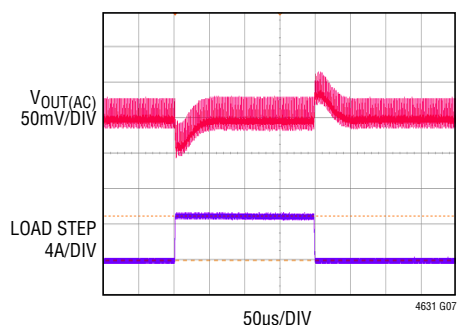
1.5V Output Single Phase Load Transient Response
