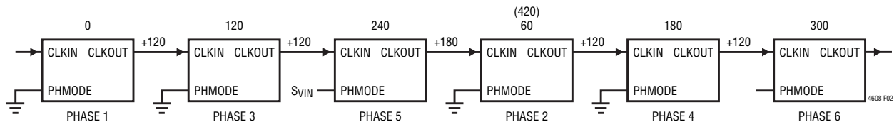
Figure 2. 6-Phase Operation
