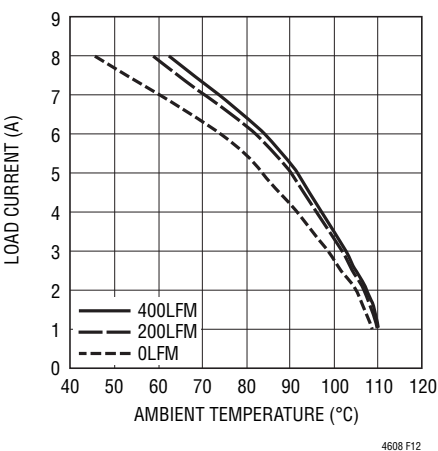
Figure 12. BGA Heat Sink with 5V IN to 1.5V OUT
