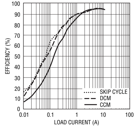
Efficiency vs Load Current 32V IN to 12V OUT
