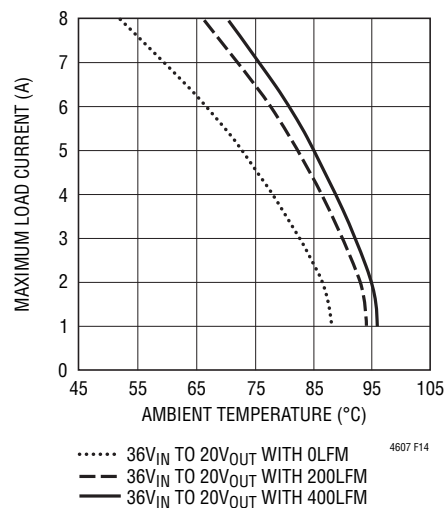
Figure 14. 36V IN to 20V OUT with Heat Sink
