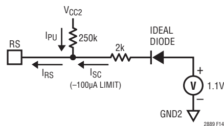
Figure 14. Equivalent Circuit of RS Pin
