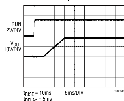
Soft-Start Ramp
