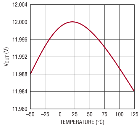
Regulated 12V Output Voltage vs Temperature
