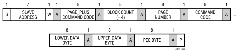
Figure 46. Example of PAGE_PLUS_WRITE
