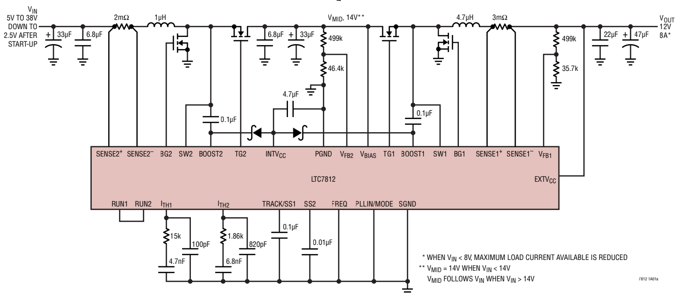
Wide Input Range to 12V/8A Low I_n , Cascaded Boost+Buck Regulator
