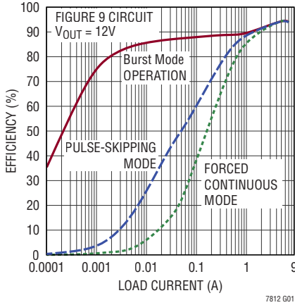
Efficiency vs Load Current V_{IN} = 9V
