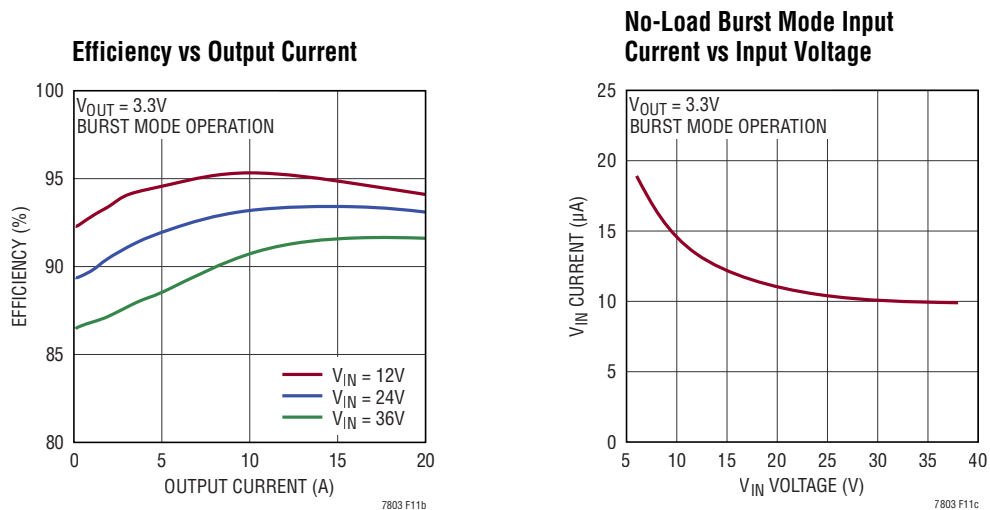
Figure 11. High Efficiency Wide Input Range 375kHz 3.3V/20A Step-Down Regulator
