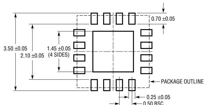
UD Package 16-Lead Plastic QFN (3mm × 3mm) (Reference LTC DWG # 05-08-1691 Rev 0)
